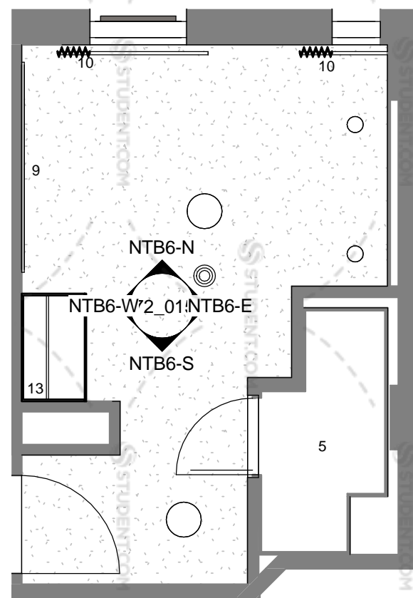
NTB6 - Reflected Ceiling Plan 1 : 50
